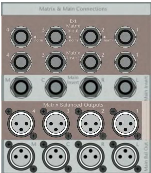
Spectra C or T Single-Point Insert Jack Unbalanced Send/Return
