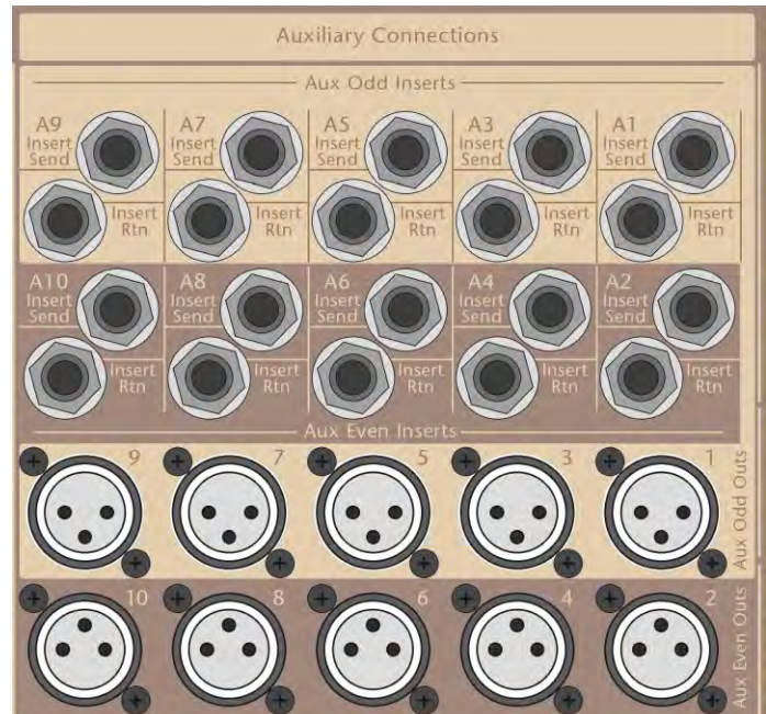
Spectra Ci or Ti Dual Insert Jacks Balanced Send/Return
