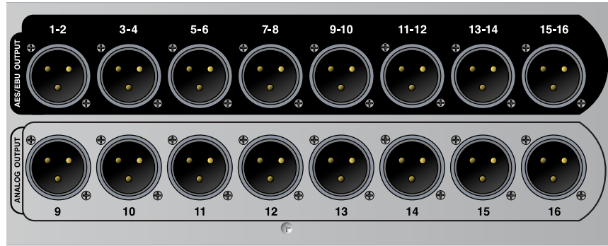
Galileo Callisto 616 AES Rear Panel Digital and Analog Outputs
