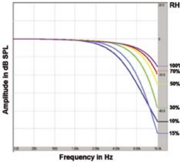
Figure i.4. Air absorption for 30 degrees C at 100 meters
