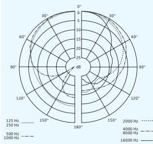
Polar diagram MMD 845-1
