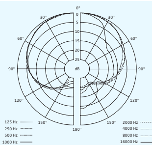
Polar diagram MME 865-1
