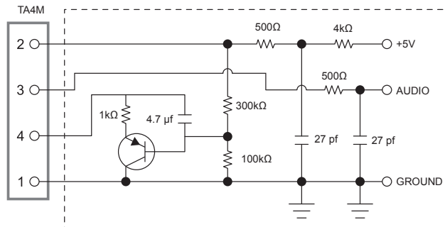
BODYPACK TRANSMITTER
