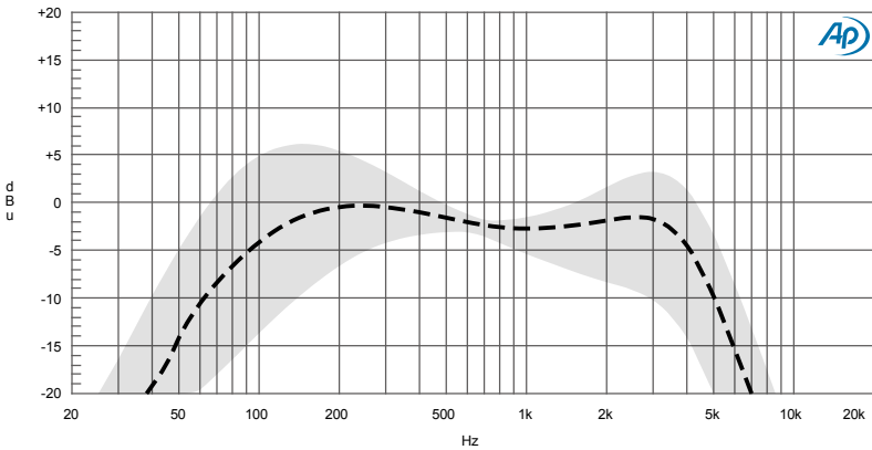
Frequency response with flat EQ settings
